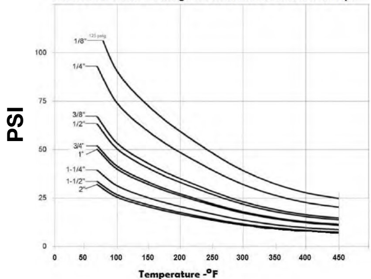
Pressure Ratings PTFE FNPT & MNPT Fittings & Connectors & Schedule 80 Pipe
